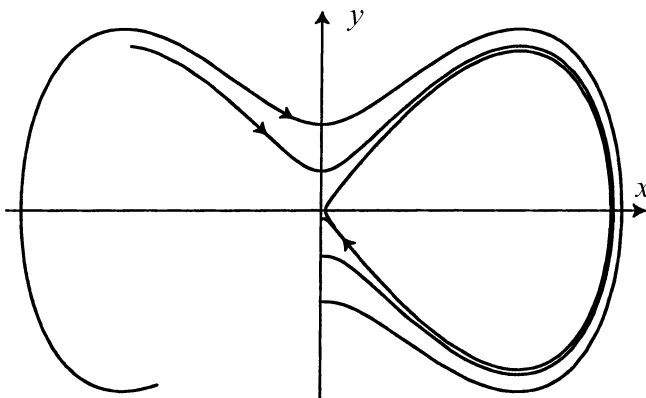
Figure 3. Phase portrait for the Brezis-Nirenberg problem after the Emden-Fowler transformation of Section 2.1 in the slightly supercritical case
