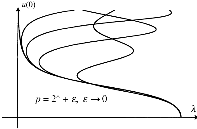
Figure 1. Bifurcation diagrams of the Brezis-Nirenberg problem (1) in the critical and slightly supercritical
