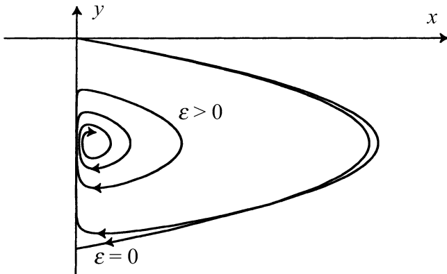
Figure 4. Phase portrait for the problem with the exponential nonlinearity after the Emden-Fowler transformation in the slightly supercritical case
