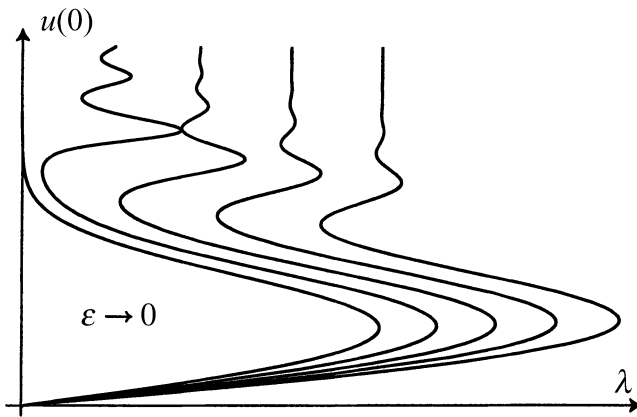
Figure 2. Bifurcation diagrams of the problem with the exponential nonlinearity (5) in the critical and slightly supercritical cases ( n = 2 , p = 2 - \epsilon ). The fact that the nonlinearity u \mapsto e^u takes a non zero value at u = 0 is responsible for the fact that the branch of minimal solutions bifurcates from (0, 0) . This is of course a fundamental difference with the Brezis-Nirenberg problem (1) which bifurcates from (\lambda_1, 0)
