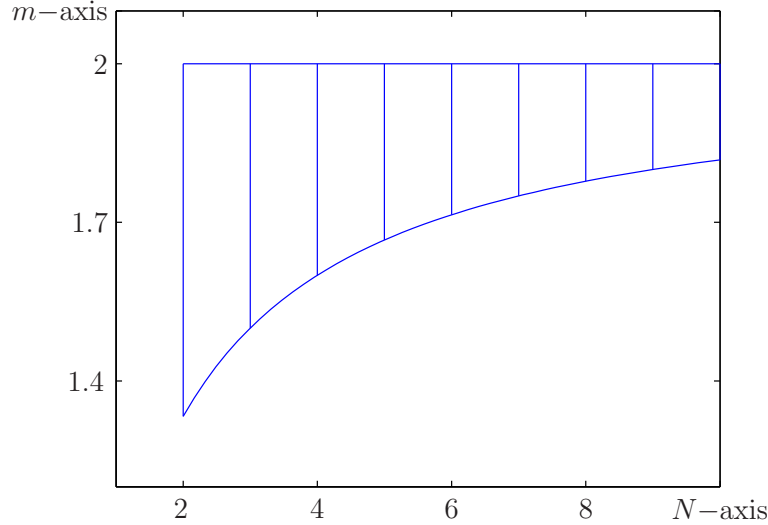
FIGURE 1. The values of m < 2 for which we obtain a new region of existence.
