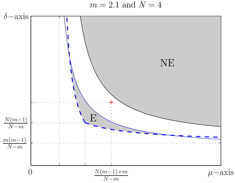
FIGURE 4. The non existence region in grey is given by (1.9). The new existence region is bounded by equality in (1.8) and the dashed curve which is given by equality (1.3).
