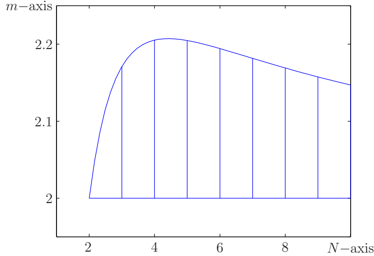
FIGURE 2. The values of m > 2 for which we obtain a new region of existence.
