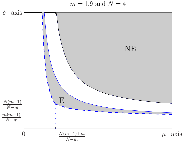
FIGURE 3. The nonexistence region in grey is given by (1.10), and the new existence region is the one bounded by equality in (1.3) and by equality in (1.6).
