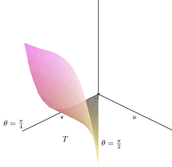
FIGURE 1. Schematic view of the function F(u, v) representing \Gamma in the sector T = \{u > 0, v > 0, u < v\} .
